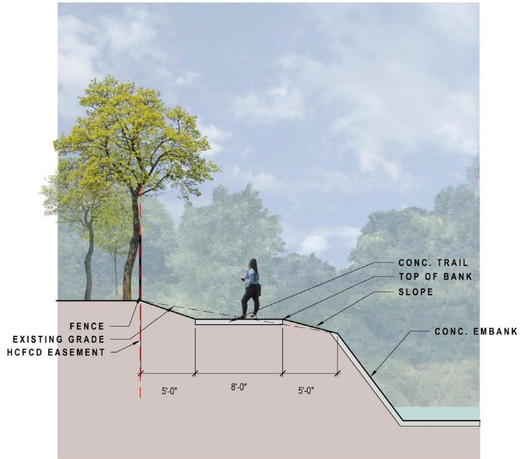
TRAIL AT NARROW CONDITION SENDERO ESTRECHO
